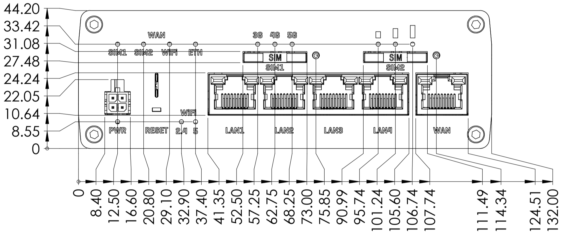
Front view
