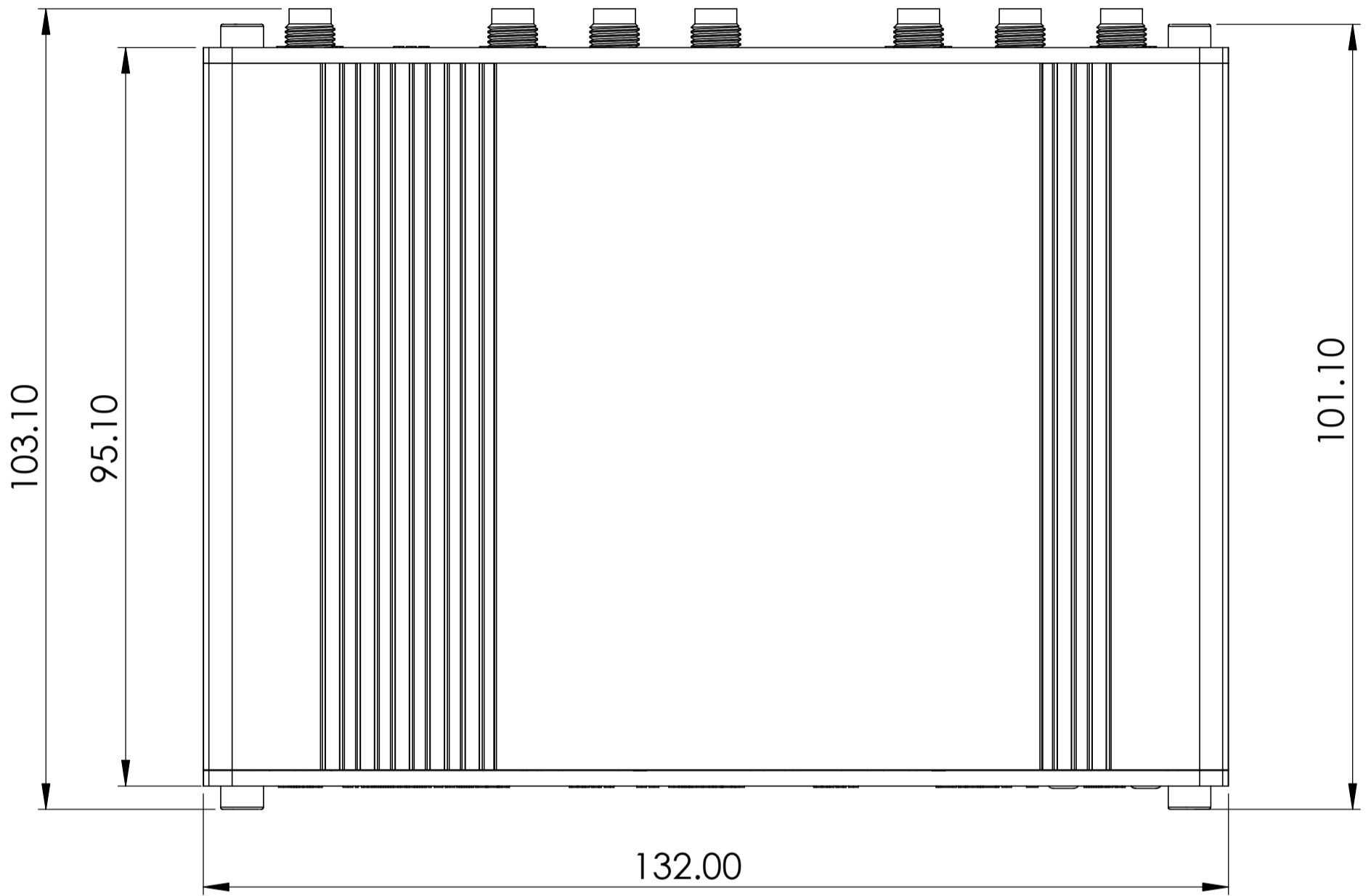
Top view
