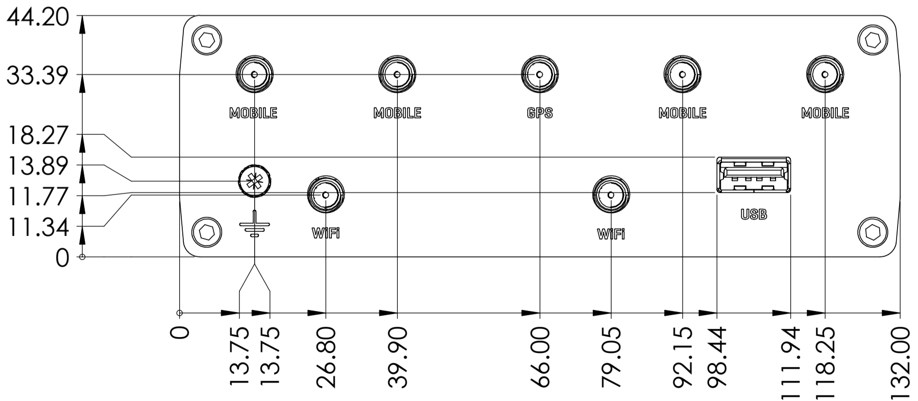
Rear view
