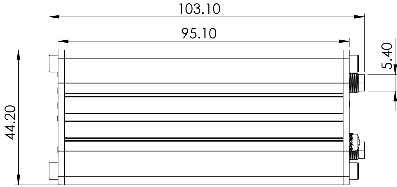
Right view
